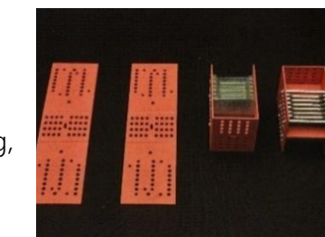
Large Stamping Parts (Size 200Φ) Outer Diameter Stamping, Grooving, Punching Bending, Platings Spot Weilding, and Caulking
