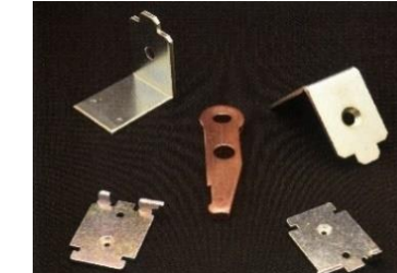
Large Stamping Parts (Size 200Φ) Outer Diameter Stamping, Grooving, Punching Bending, Platings Spot Weilding, and Caulking
